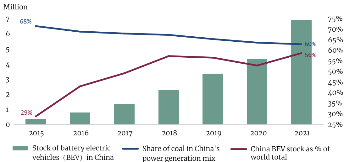
Figure 8. Share of coal power in China's power mix and rising deployment of battery EVs in China, 2015-2021
