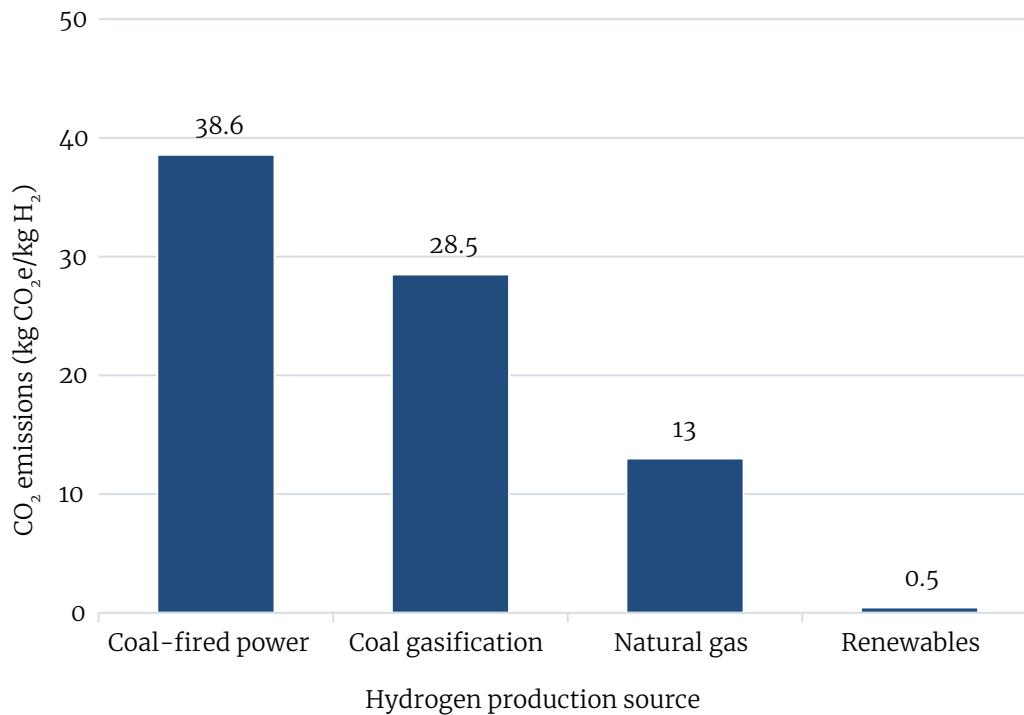
Figure 4. CO 2 intensity of hydrogen production in China (kg CO 2 e/kg H 2 )
